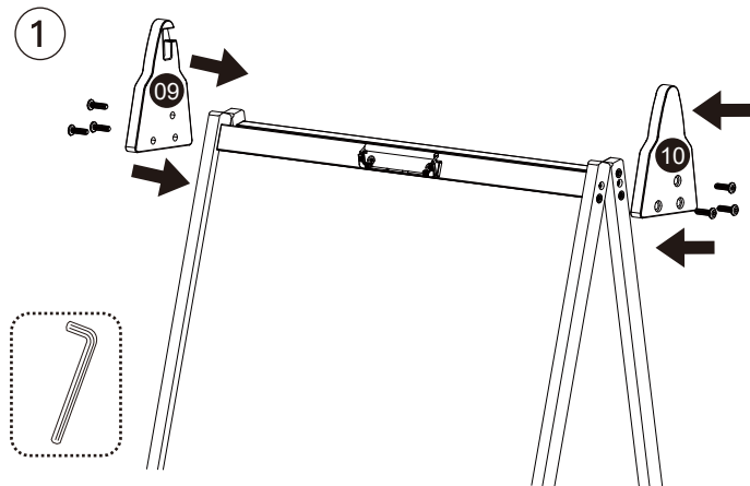
09 Left Ear*1 10 Right Ear*1 11 Screws A*6
